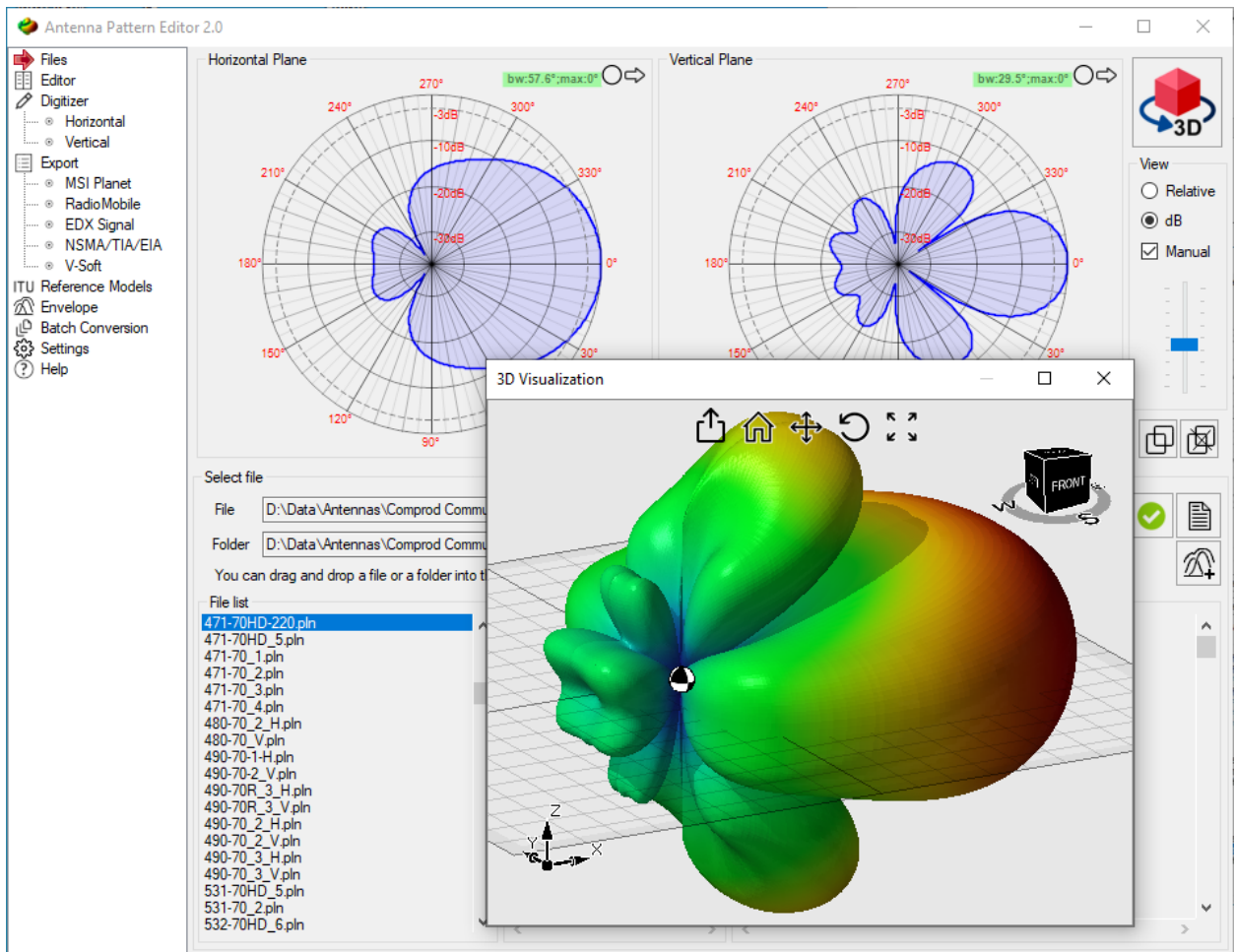
3D visualization of 2D antenna pattern
