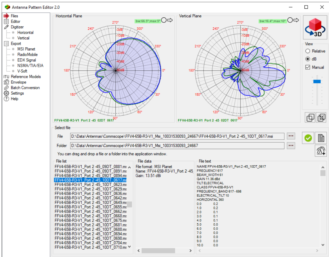
Comparison of two antenna patterns
