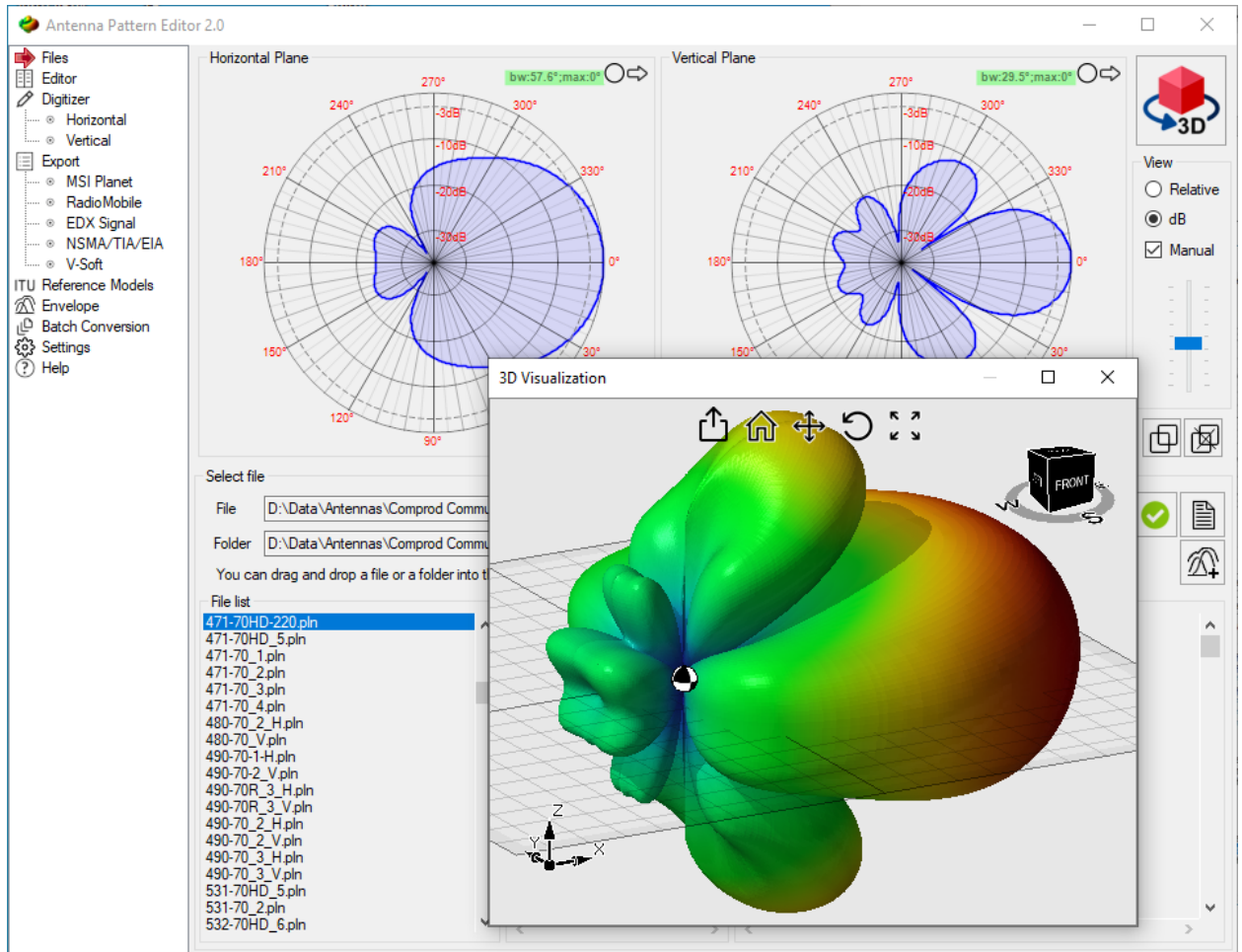
3D visualization of 2D antenna pattern
