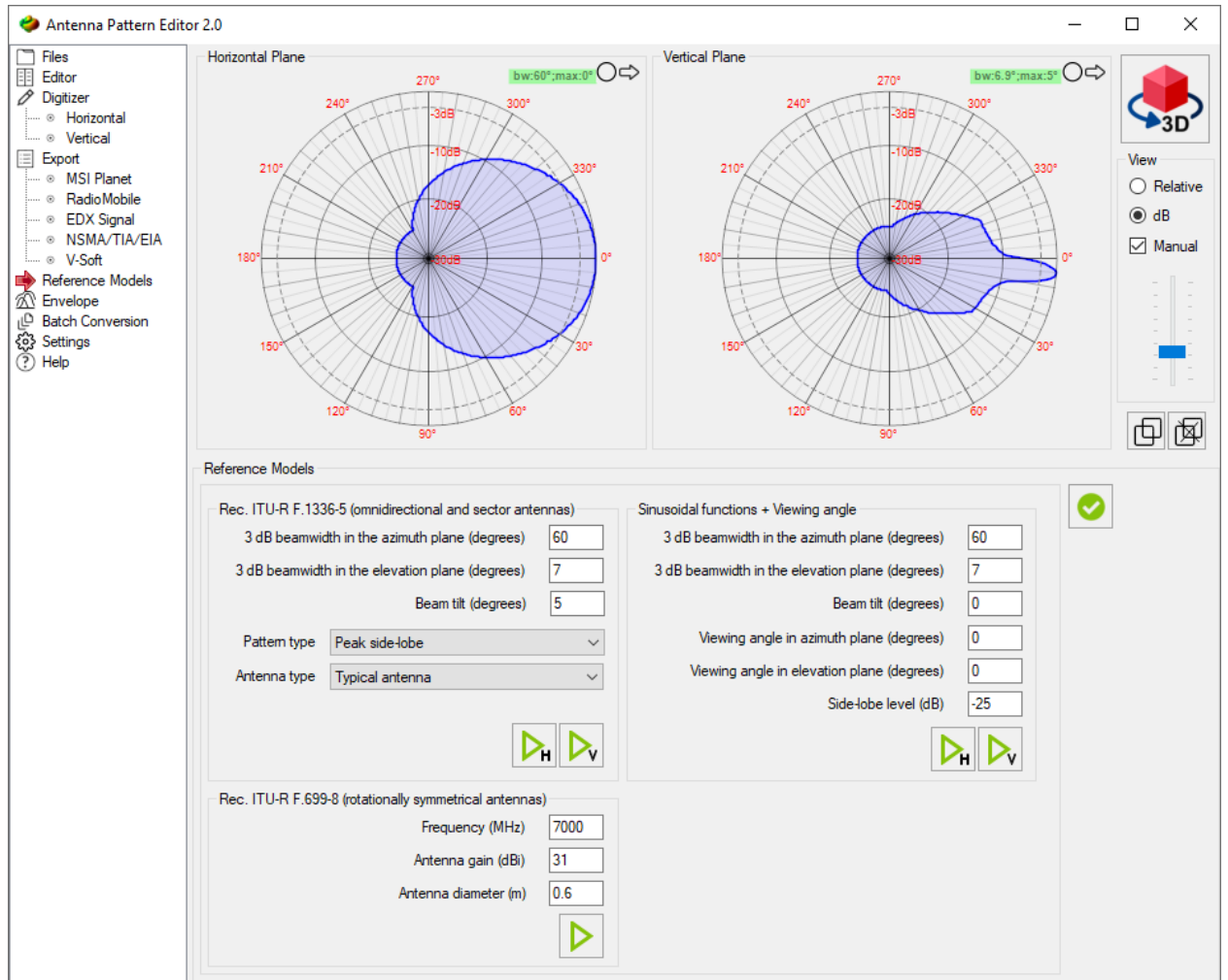
Antenna Pattern Synthesis by Reference Models
