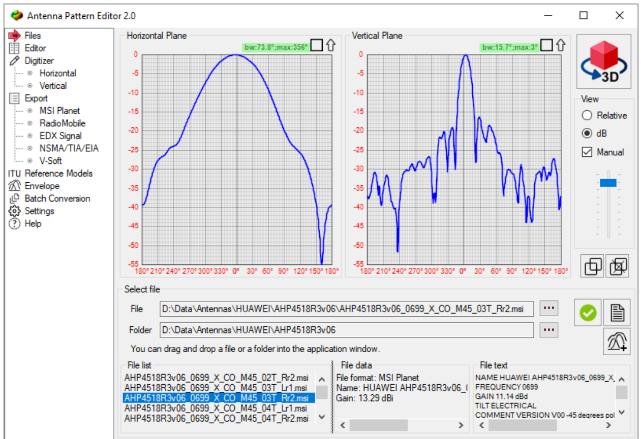
Antenna Pattern in Cartesian Coordinate System
